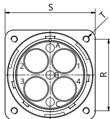
Size 40 and module number I4
