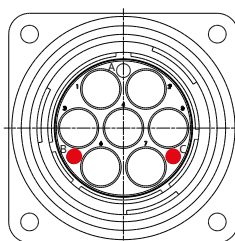
Size 48 and module number A7/I7
