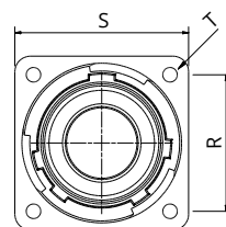
Size 24 and module number A1/I1
