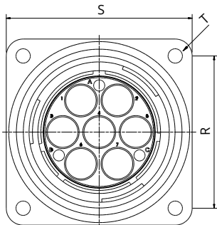
Size 48 and module number A7/I7
